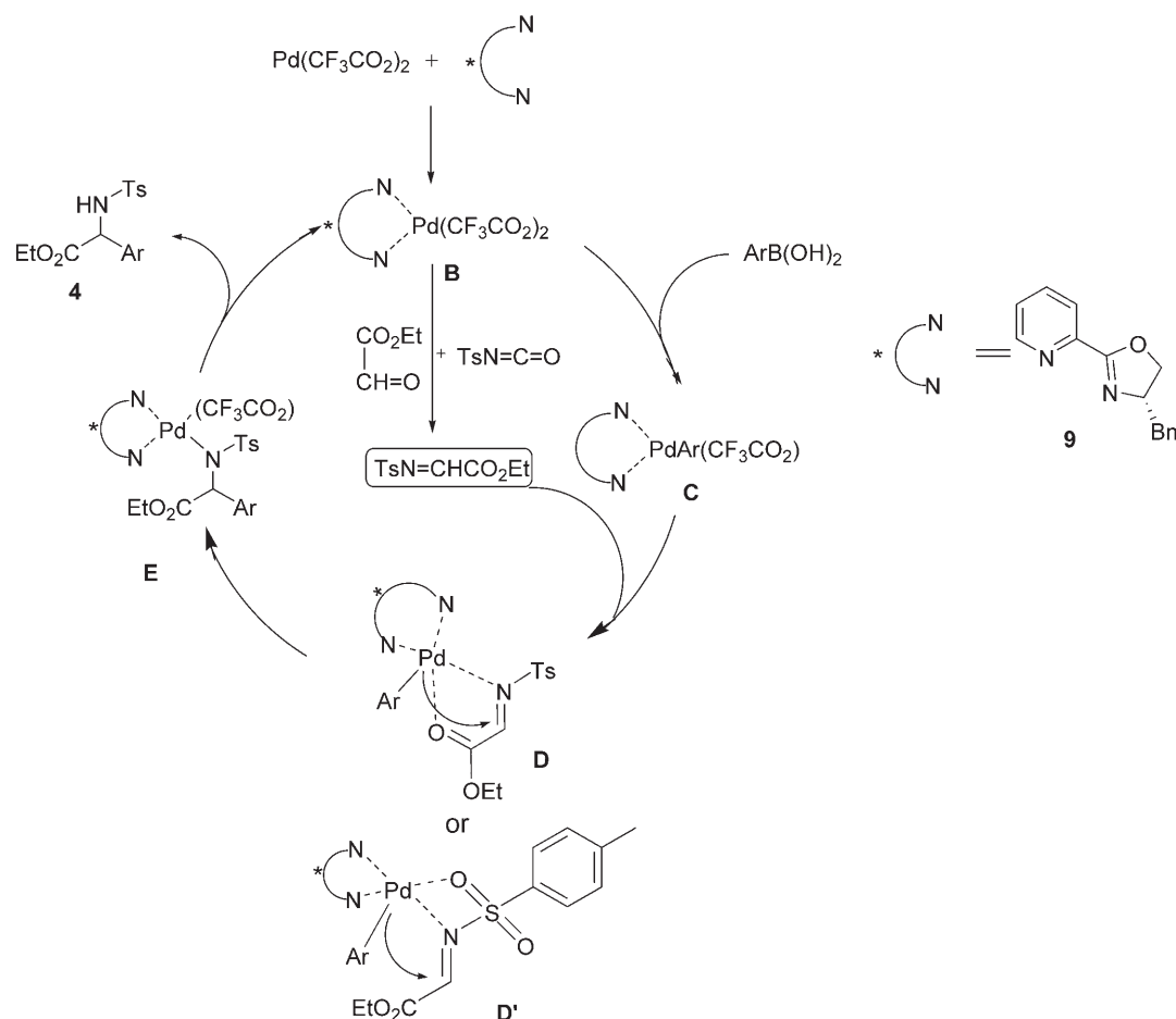
Scheme 3. Proposed mechanism for the palladium(II)-catalyzed one-pot enantioselective synthesis of arylglycines from ethyl glyoxylate, p -toluenesulfonyl isocyanate and arylboronic acids.
