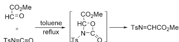
Scheme 1. Formation of imino esters from p -toluenesulfonyl isocyanate and methyl glyoxylate.
