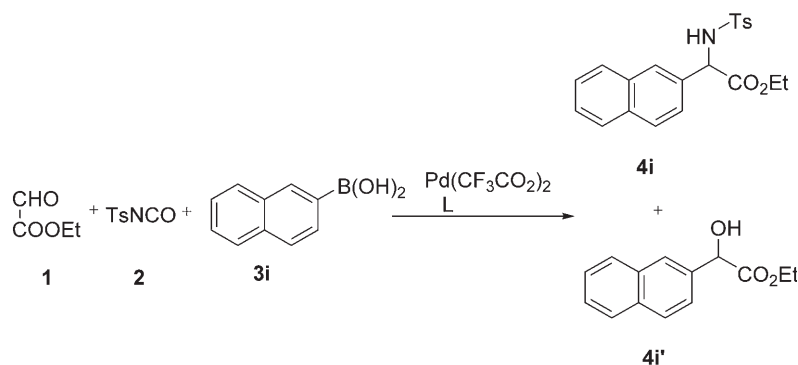
Scheme 2. Formation of a by-product from β-naphthylboronic acid.
